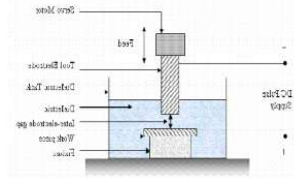
Figure 1. Principle of EDM
